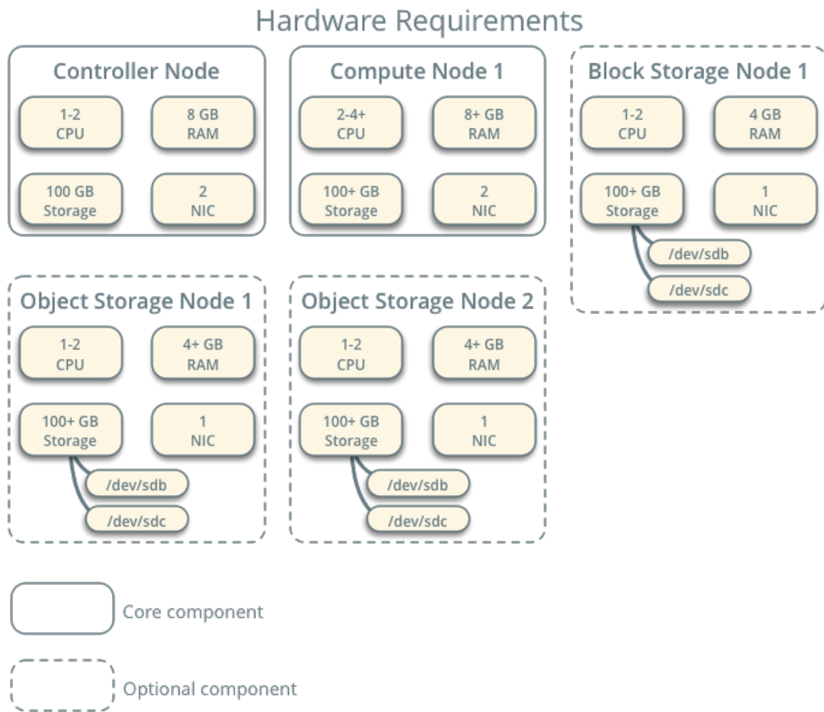
Fig. 1: Hardware requirements
