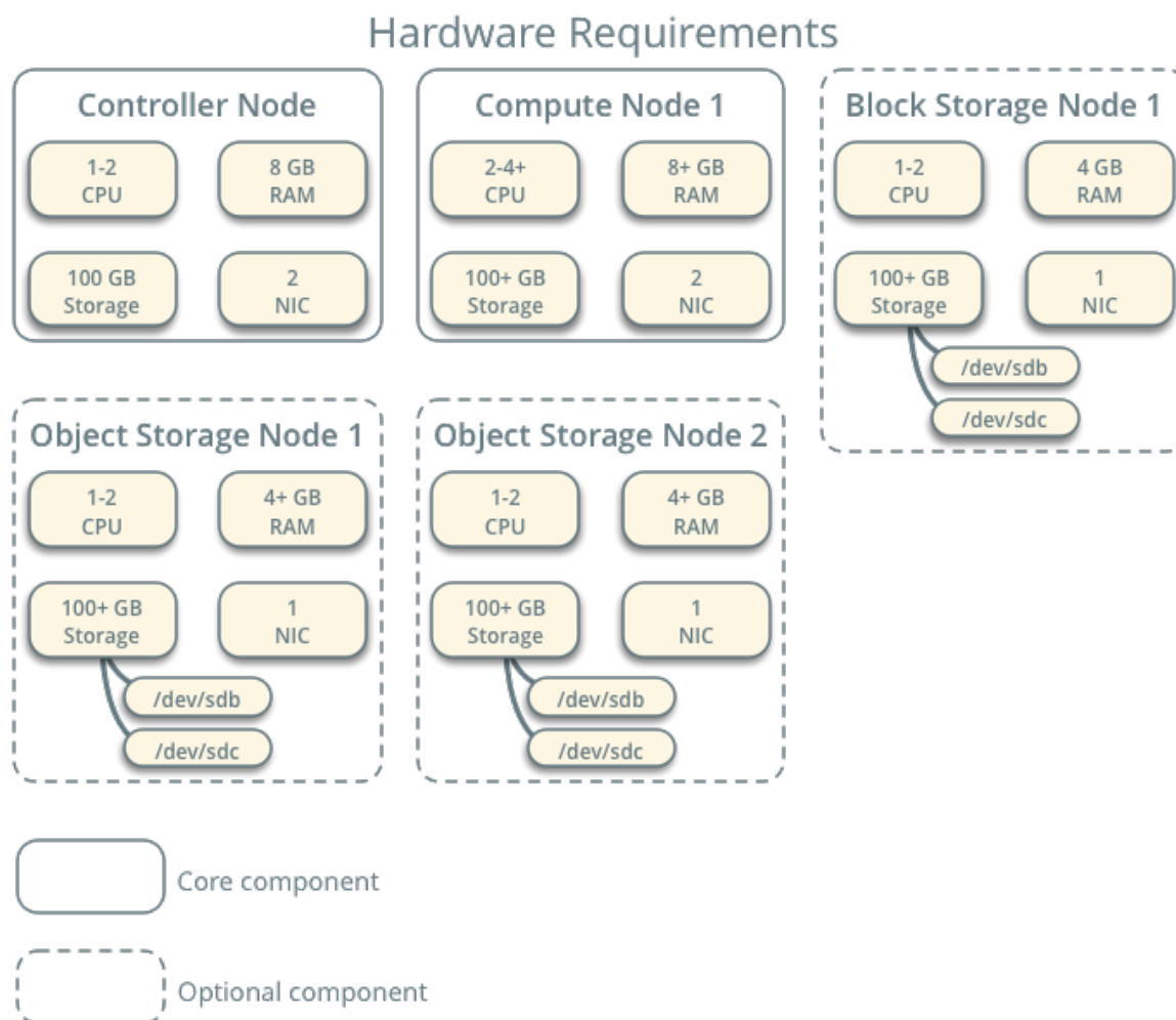
Fig. 1: Hardware requirements
