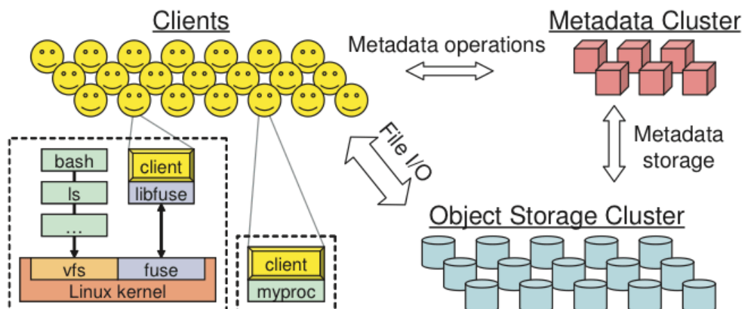
Fig. 1: Ceph architecture
